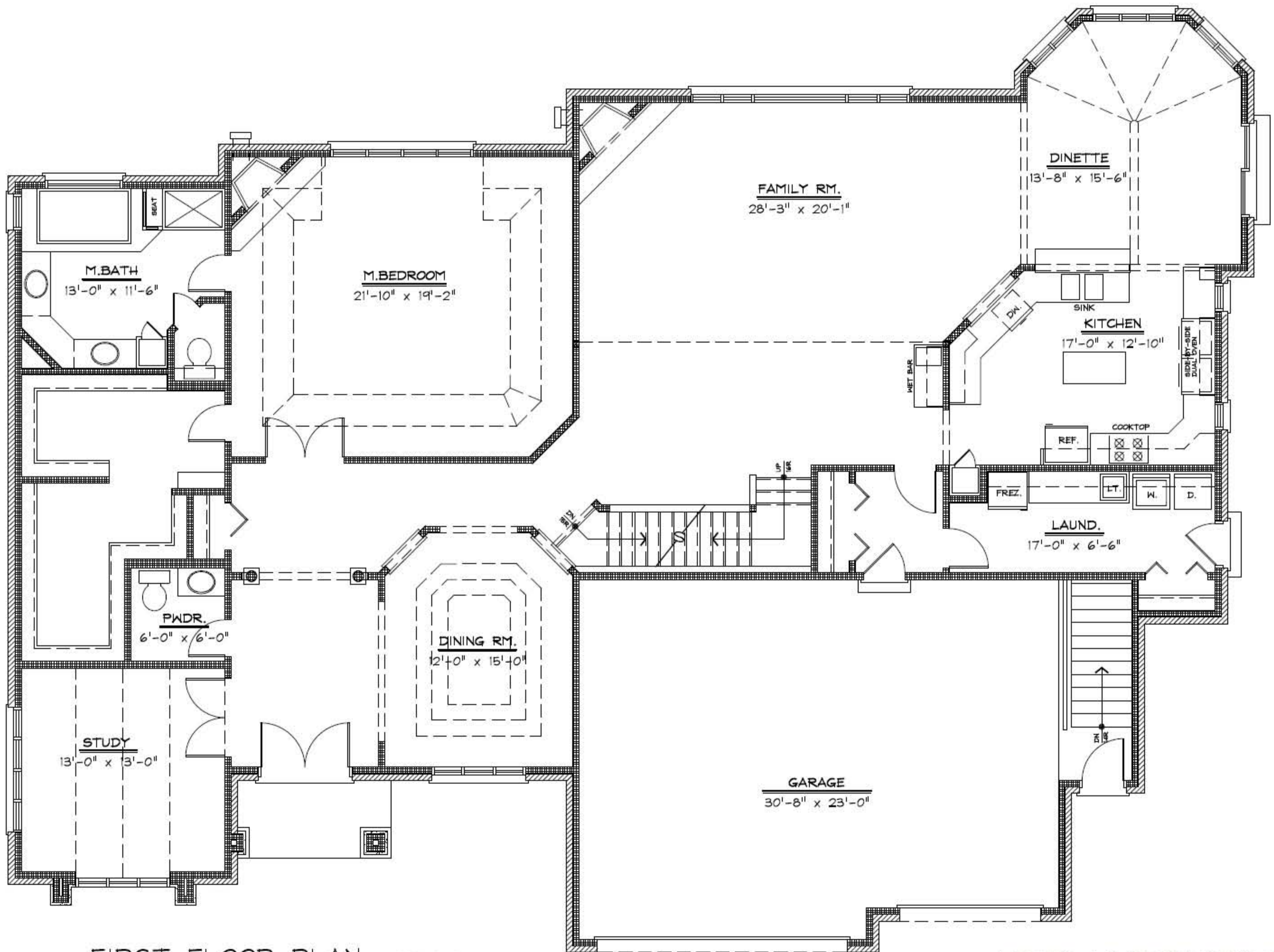
FIRST FLOOR PLAN 2926 S.F. ADAIR ARCHITECTS PLAN #0009
