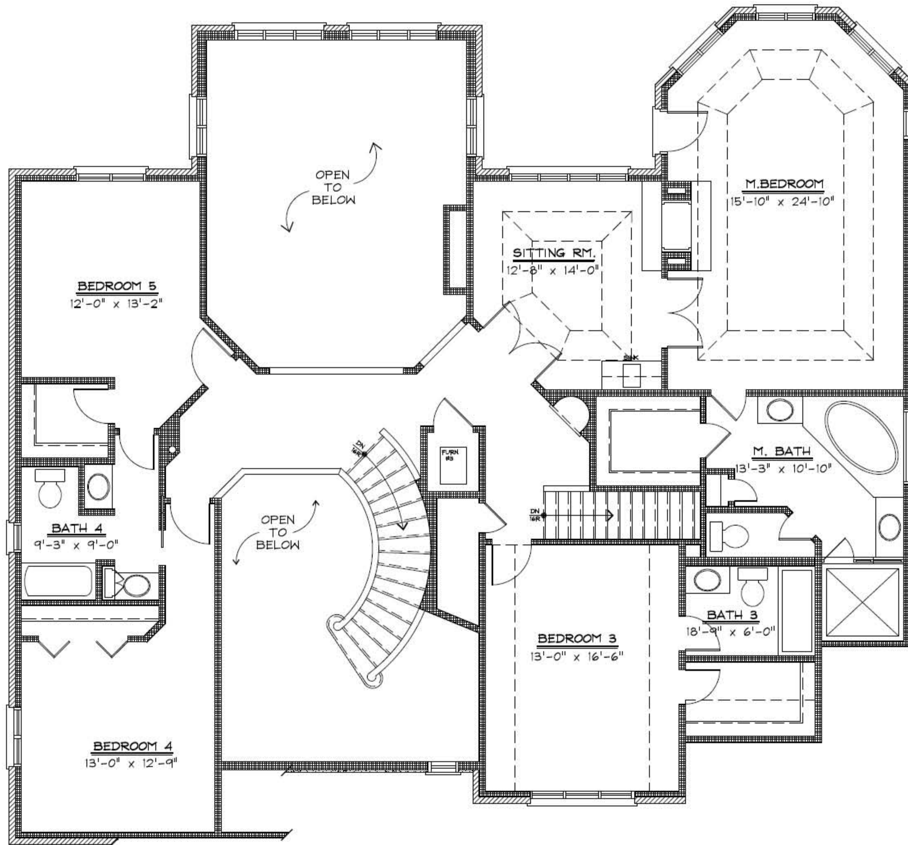
SECOND FLOOR PLAN 2193 S.F. ADAIR ARCHITECTS PLAN #0015
