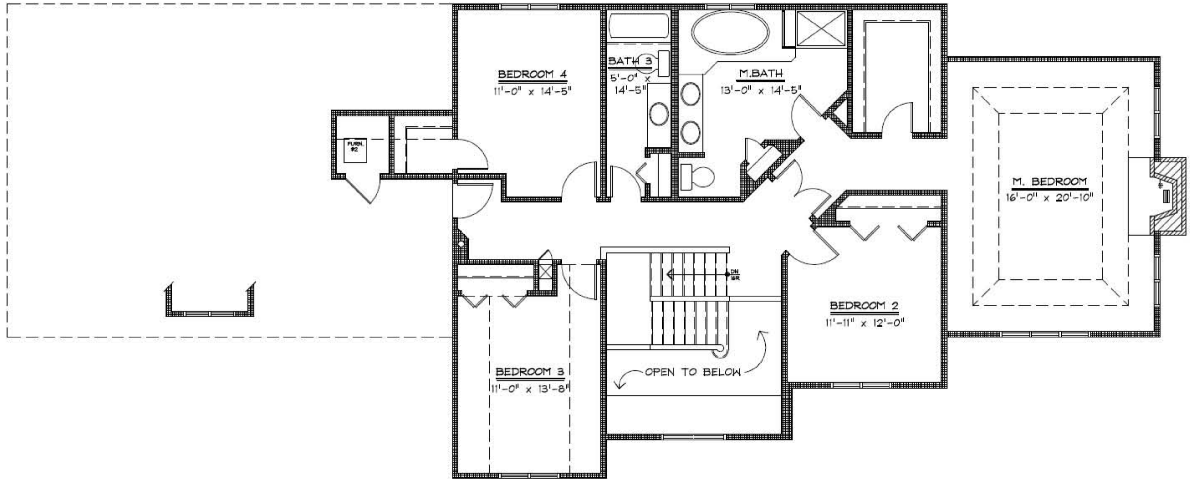
SECOND FLOOR PLAN 1438 S.F. ADAIR ARCHITECTS PLAN #0109
