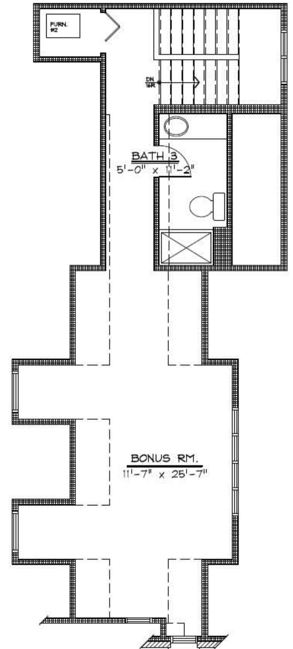
BONUS RM. FLOOR PLAN ADAIR ARCHITECTS PLAN #0215
