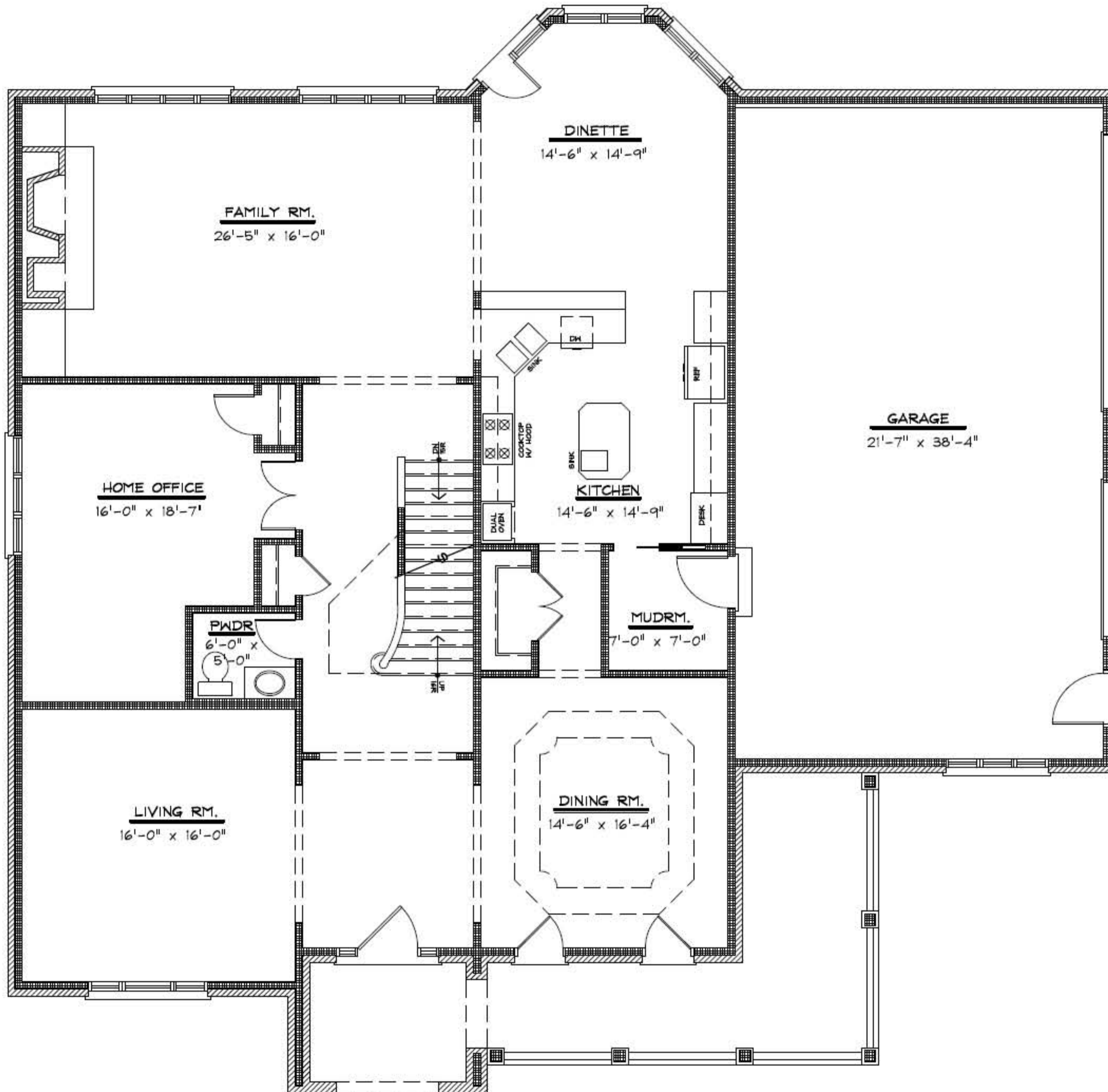
FIRST FLOOR PLAN 2286 S.F. ADAIR ARCHITECTS PLAN #0306
