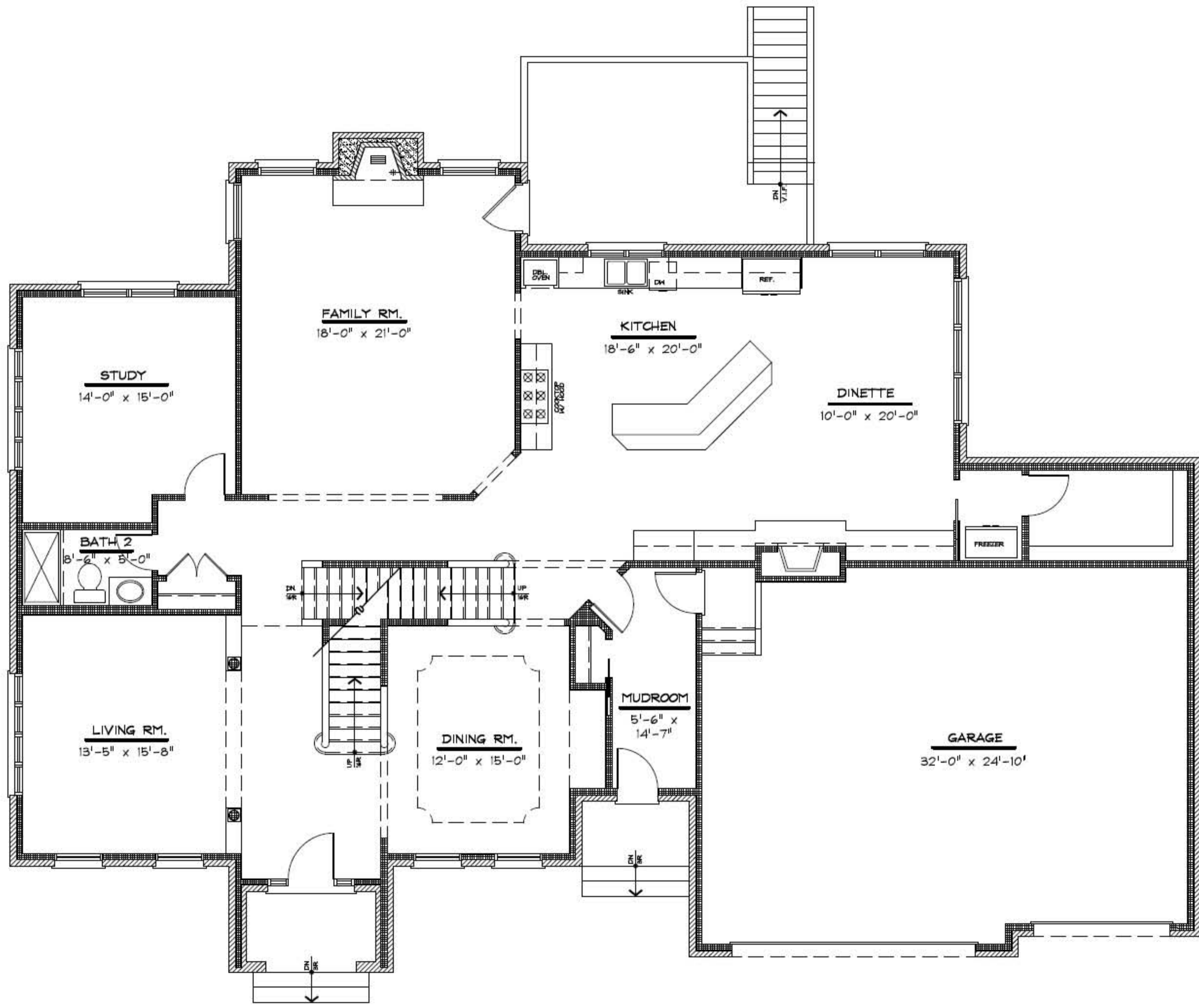
FIRST FLOOR PLAN 2400 S.F. ADAIR ARCHITECTS PLAN #0316-E
