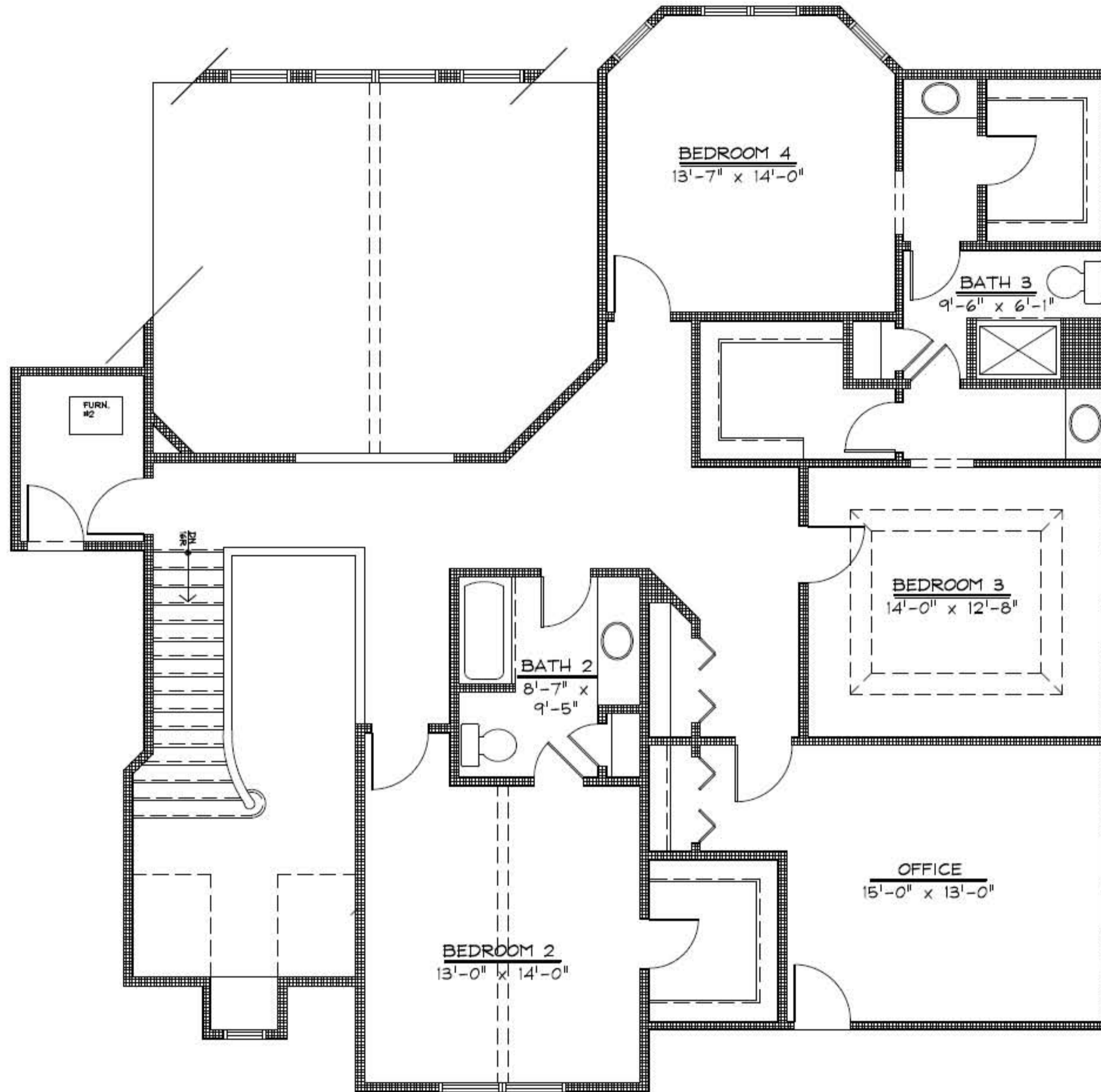
SECOND FLOOR PLAN 1597 S.F. ADAIR ARCHITECTS PLAN #0403
