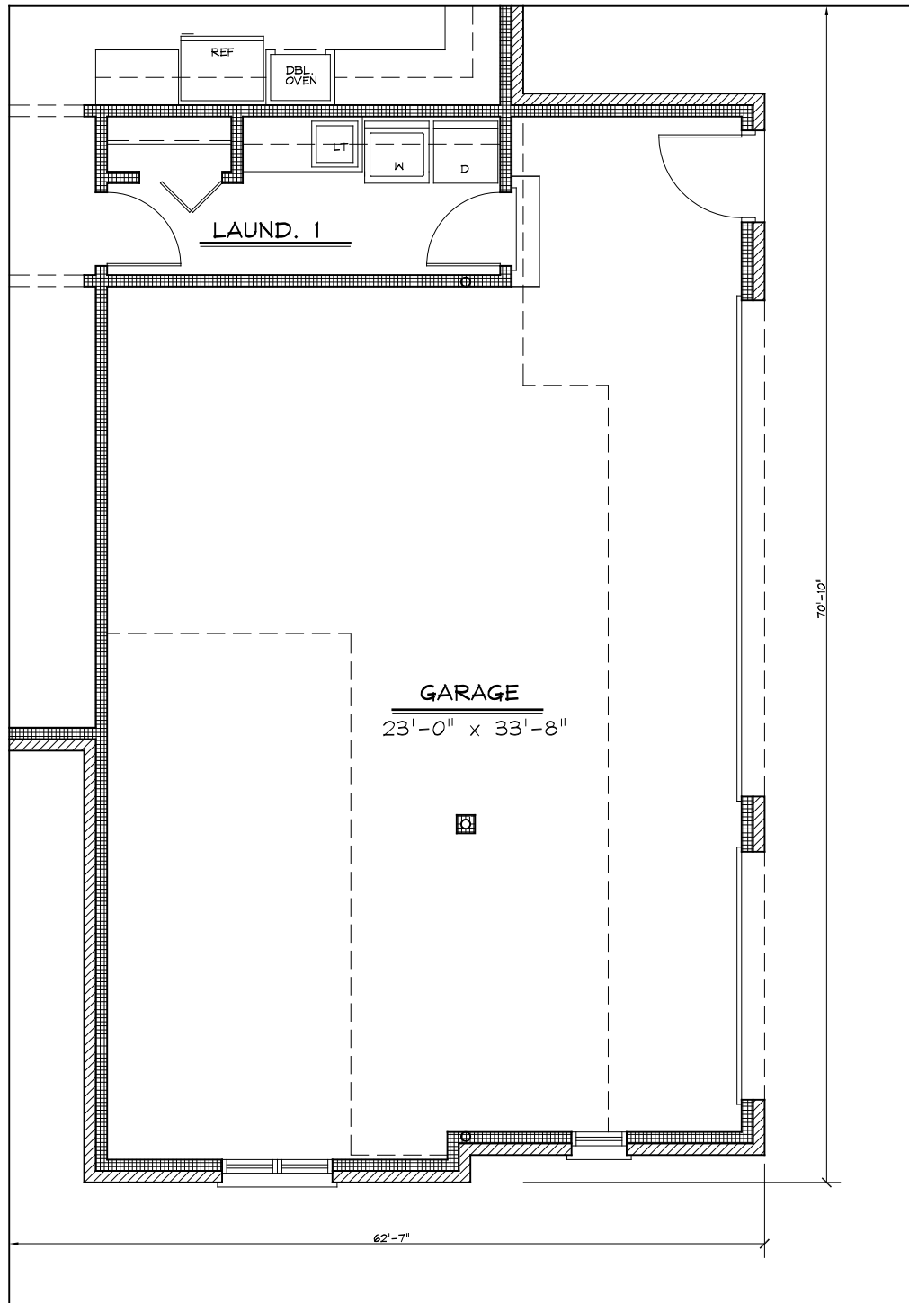
ALT. FIRST FLOOR PLAN
