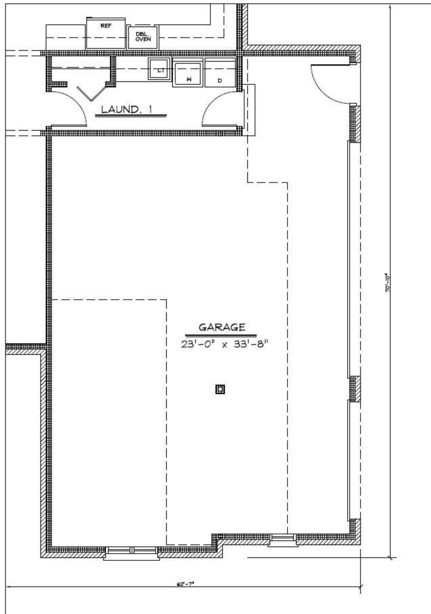
ALT. FIRST FLOOR PLAN
