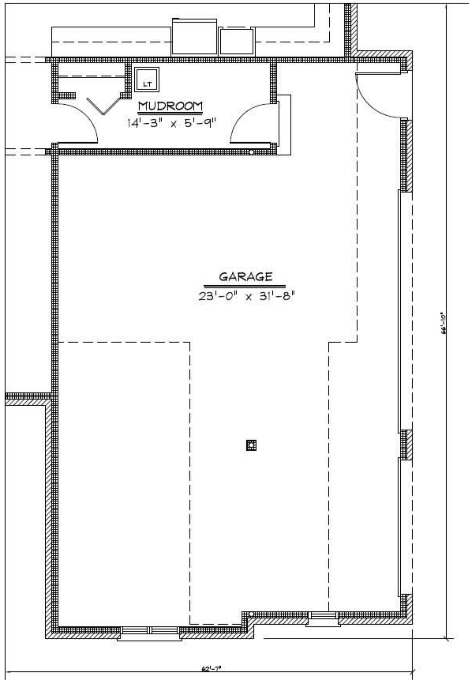
ALT. FIRST FLOOR PLAN
