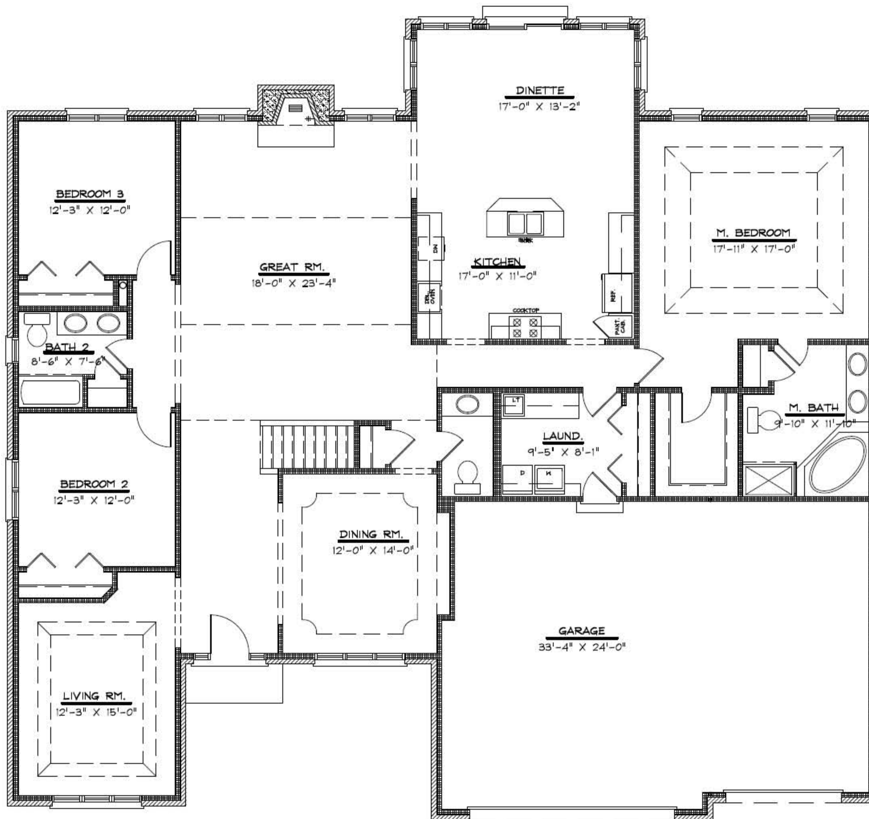
FIRST FLOOR PLAN 2803 S.F. ADAIR ARCHITECTS PLAN #0406-2
