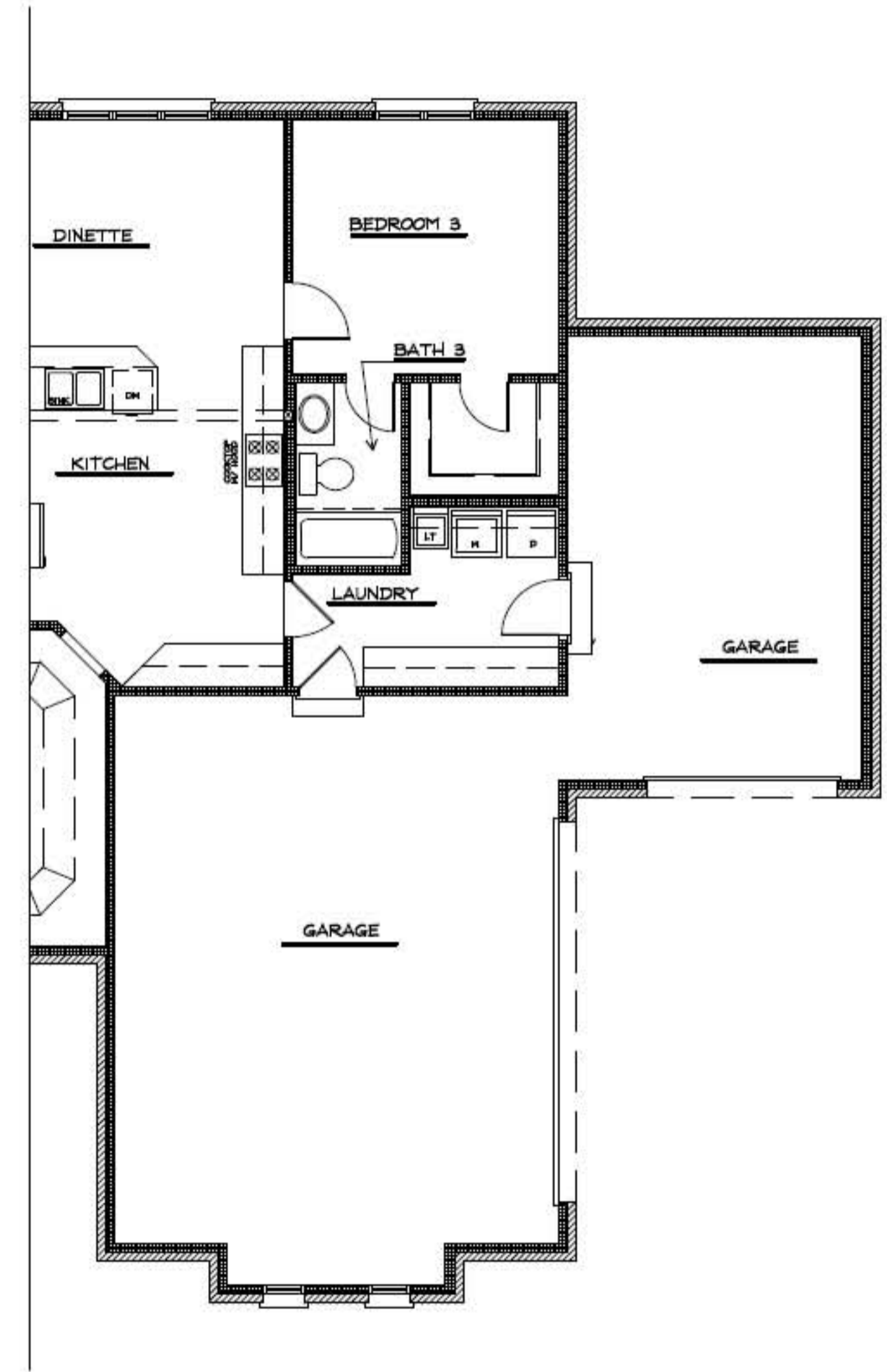
PART. FIRST FLR. PLAN W/ ALT. 3 CAR ADAIR ARCHITECTS PLAN #0418
