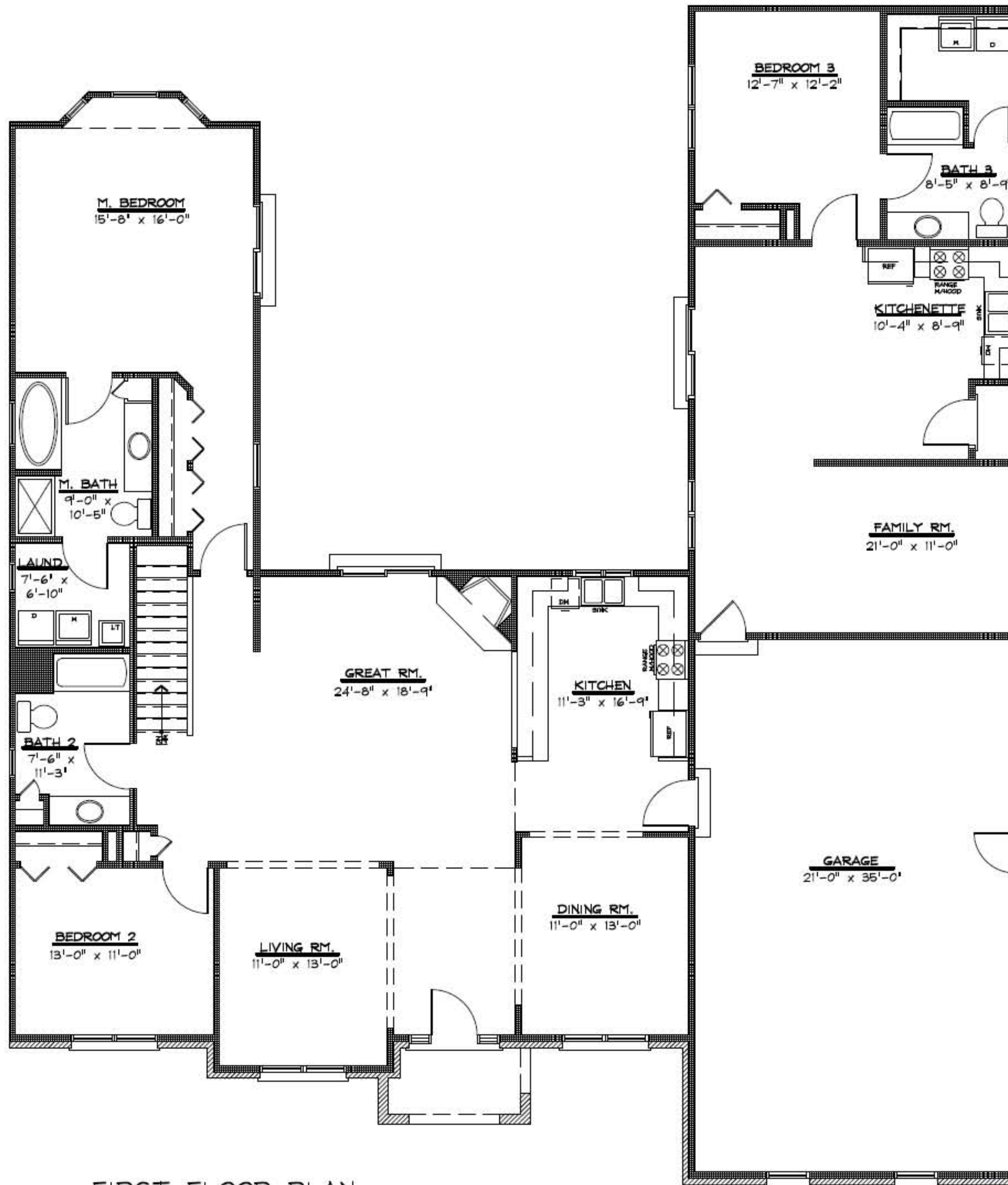
FIRST FLOOR PLAN 2850 S.F. ADAIR ARCHITECTS PLAN #0512
