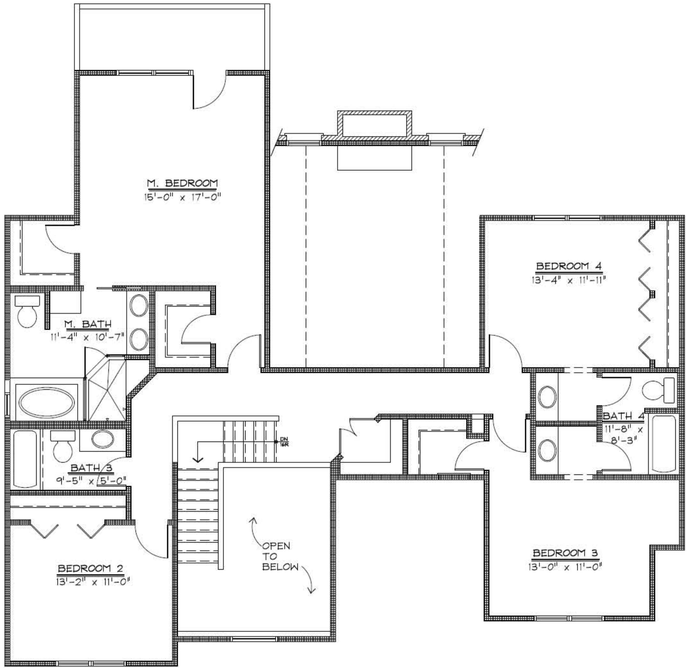
SECOND FLOOR PLAN 1467 S.F. ADAIR ARCHITECTS PLAN #0515
