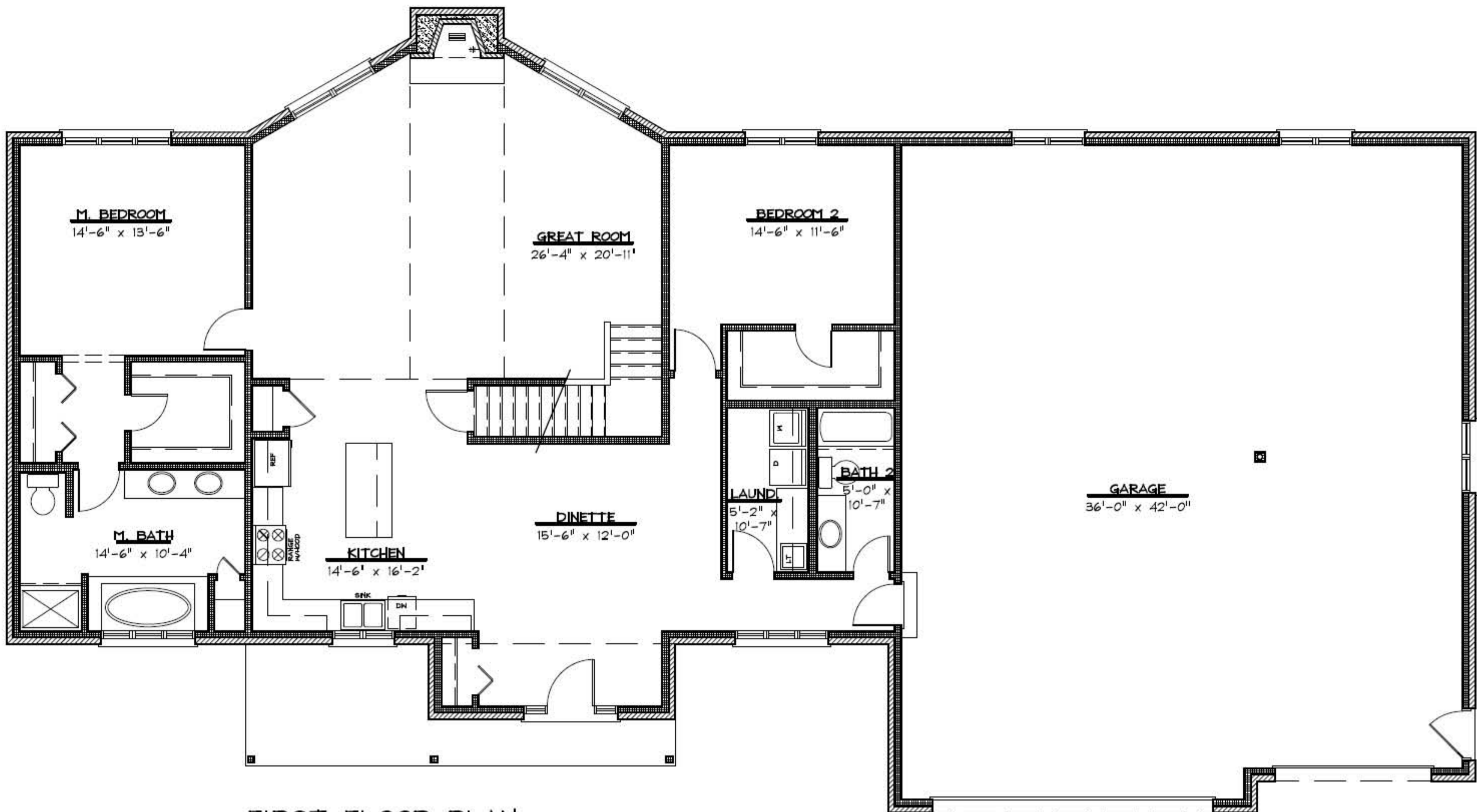
FIRST FLOOR PLAN 2440 S.F.
