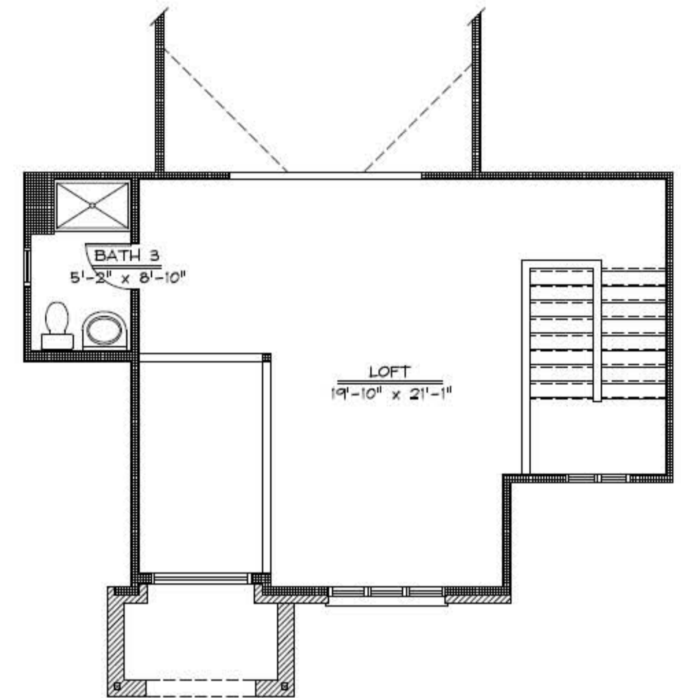
LOFT FLOOR PLAN
