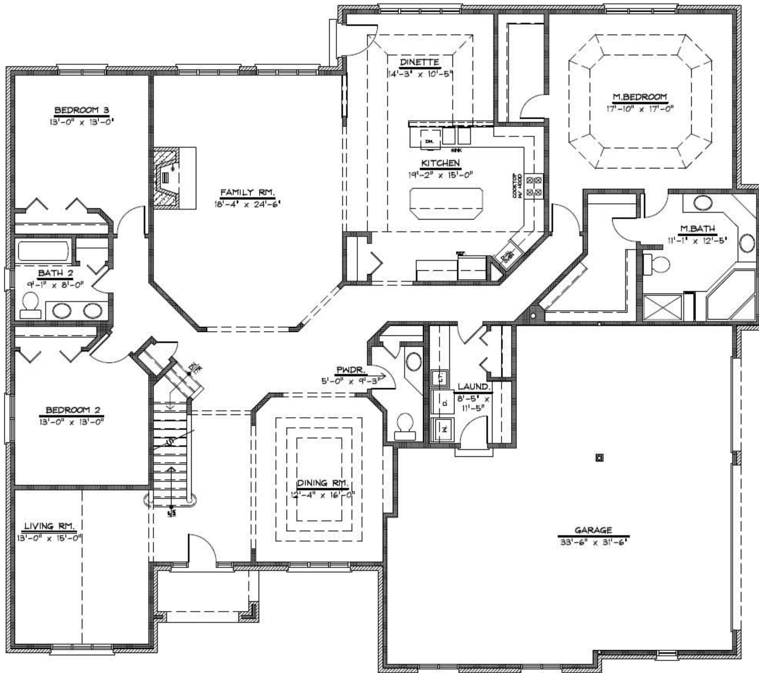
FIRST FLOOR PLAN 3702 S.F. ADAIR ARCHITECTS PLAN # 9907-3
