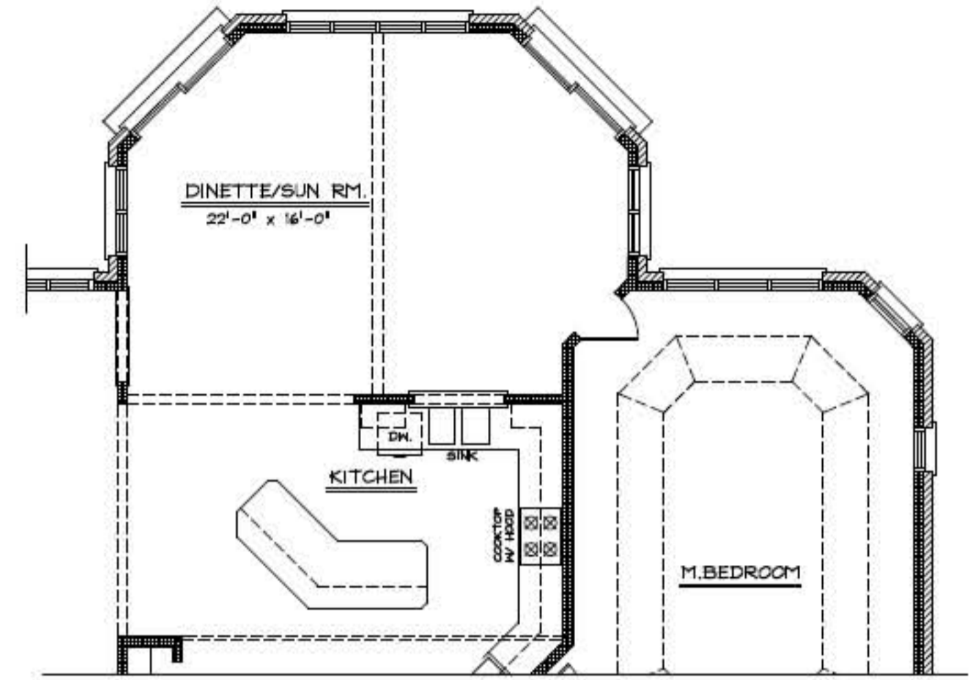
ALTERNATE SUNROOM FLOOR PLAN ADAIR ARCHITECTS PLAN # 9907-C
